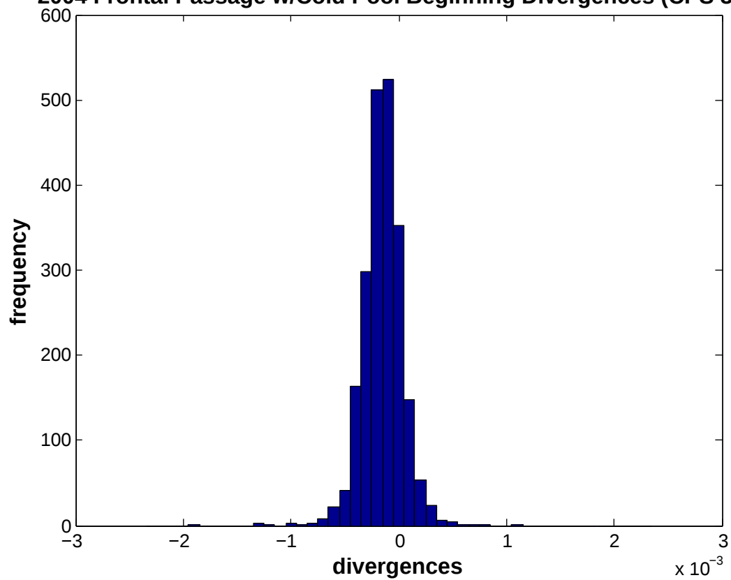
2004 Frontal Passage w/Cold Pool Beginning Divergences (CPS 3+)
