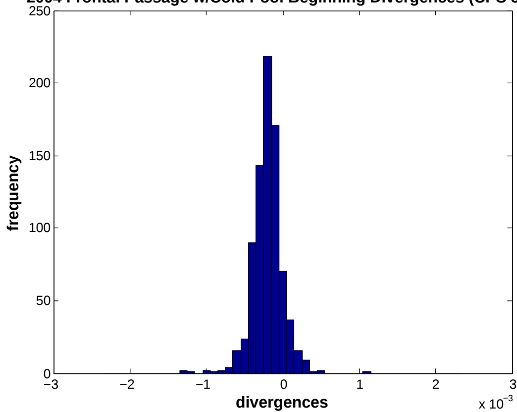
2004 Frontal Passage w/Cold Pool Beginning Divergences (CPS 5+)
