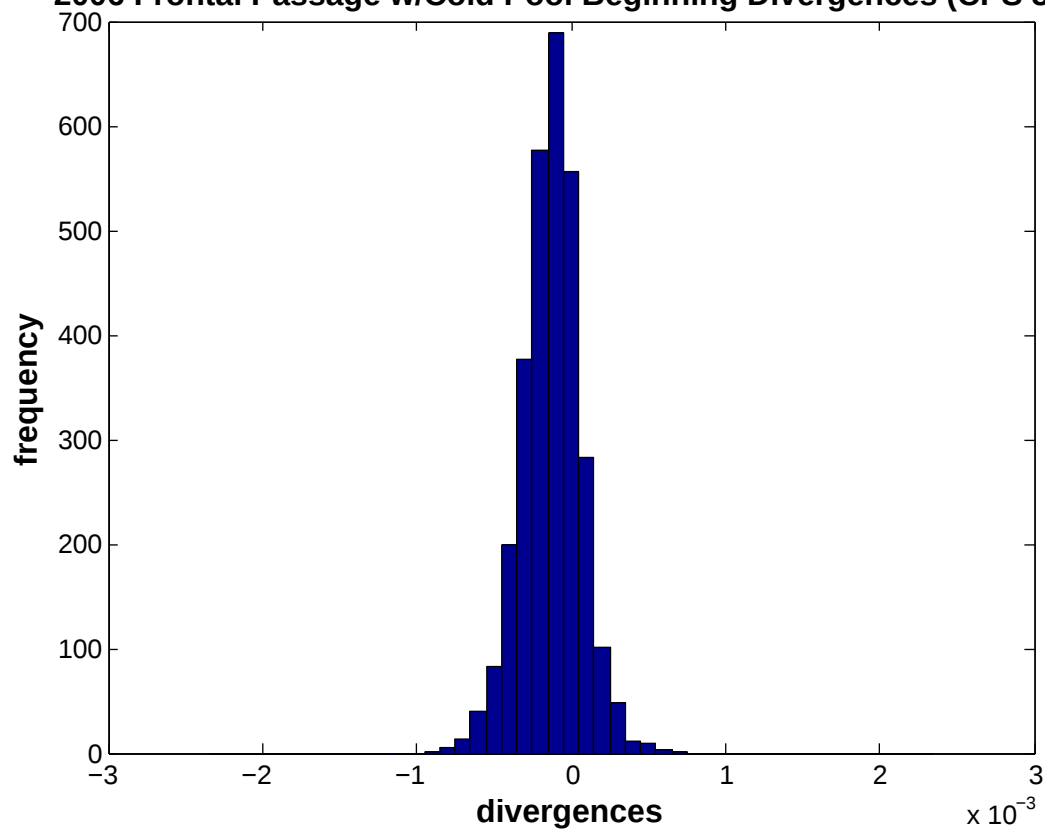
2006 Frontal Passage w/Cold Pool Beginning Divergences (CPS 3+)
