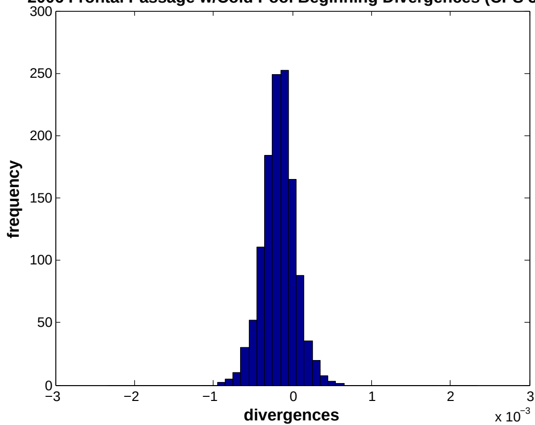
2006 Frontal Passage w/Cold Pool Beginning Divergences (CPS 5+)
