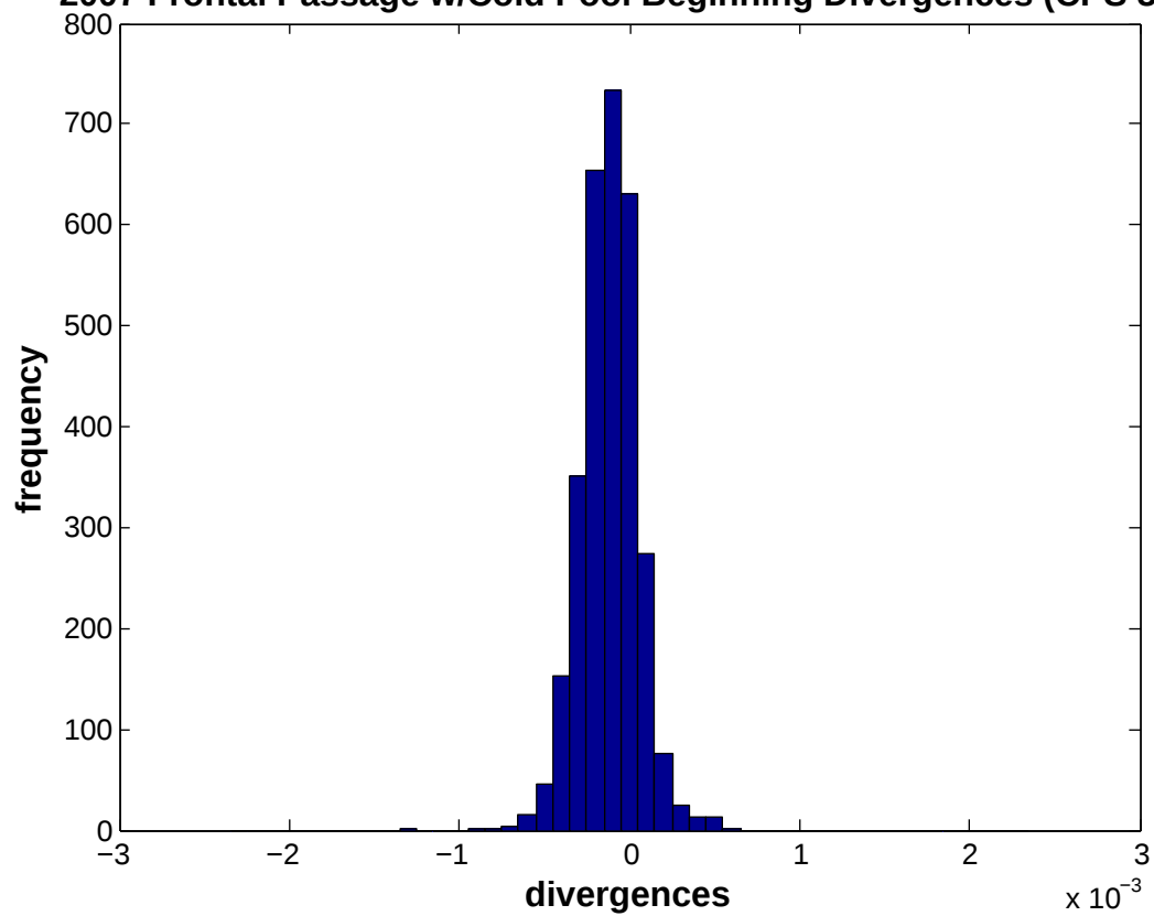
2007 Frontal Passage w/Cold Pool Beginning Divergences (CPS 3+)
