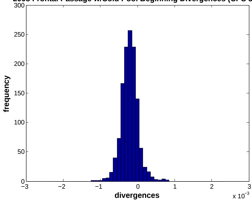
2008 Frontal Passage w/Cold Pool Beginning Divergences (CPS 5+)
