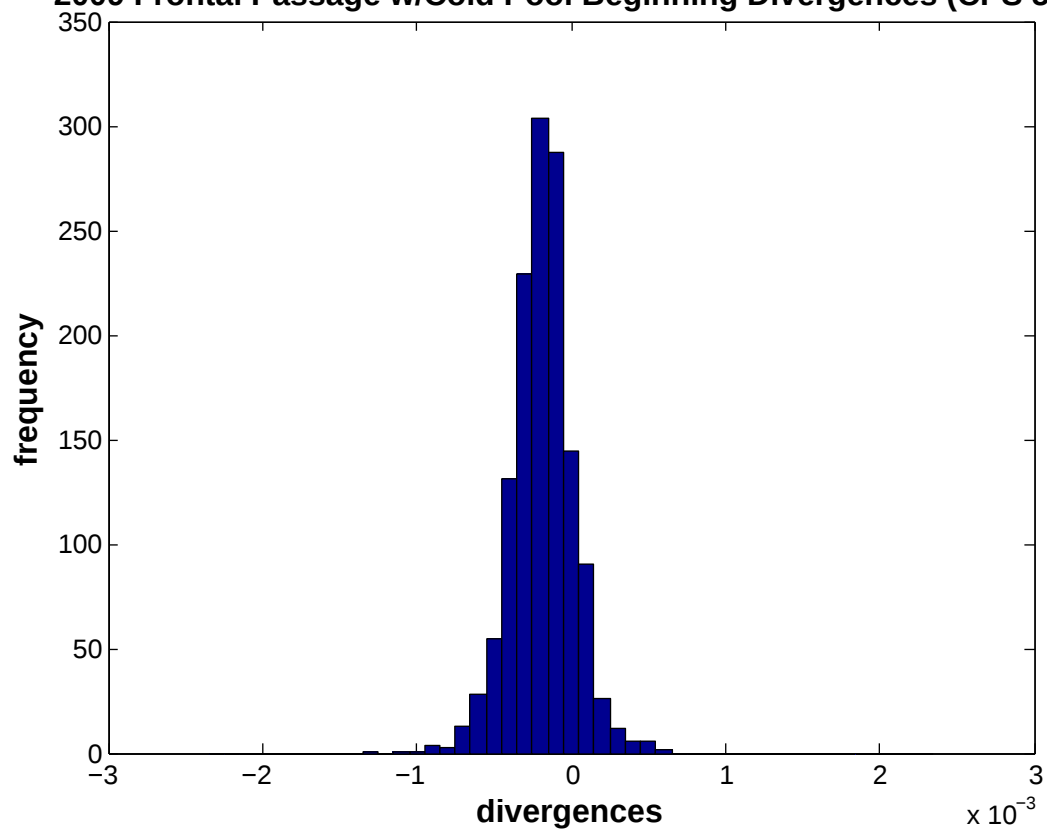
2009 Frontal Passage w/Cold Pool Beginning Divergences (CPS 5+)
