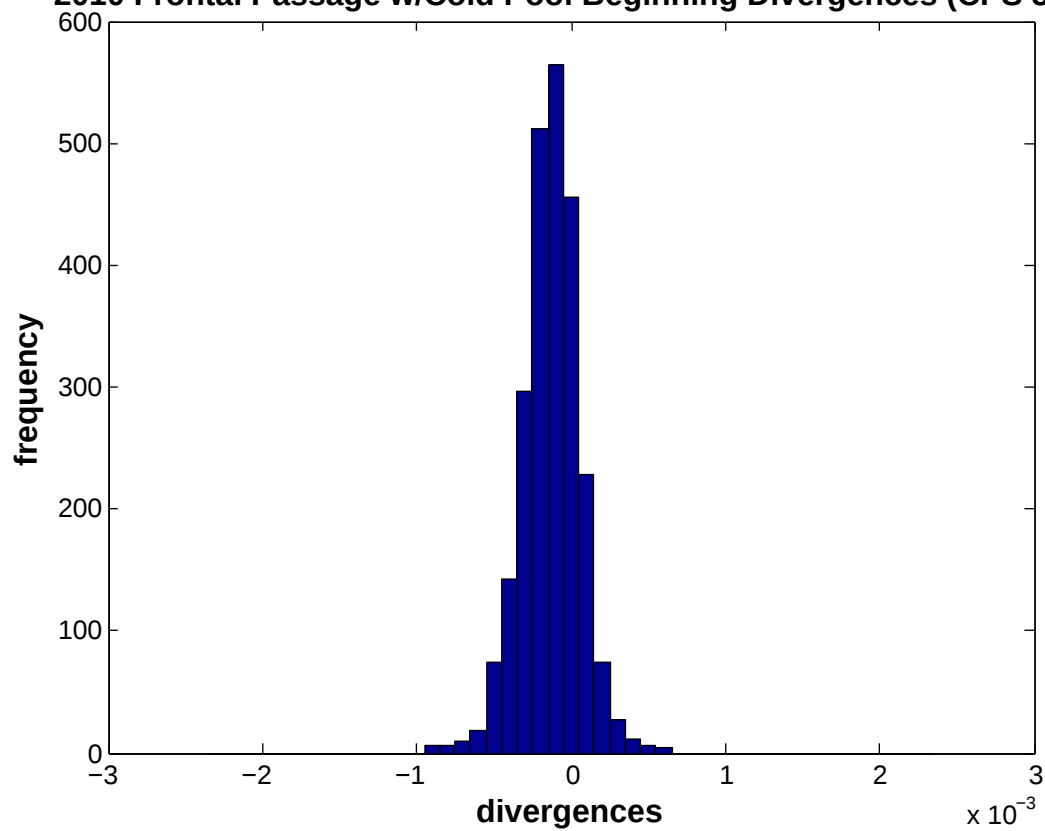
2010 Frontal Passage w/Cold Pool Beginning Divergences (CPS 3+)
