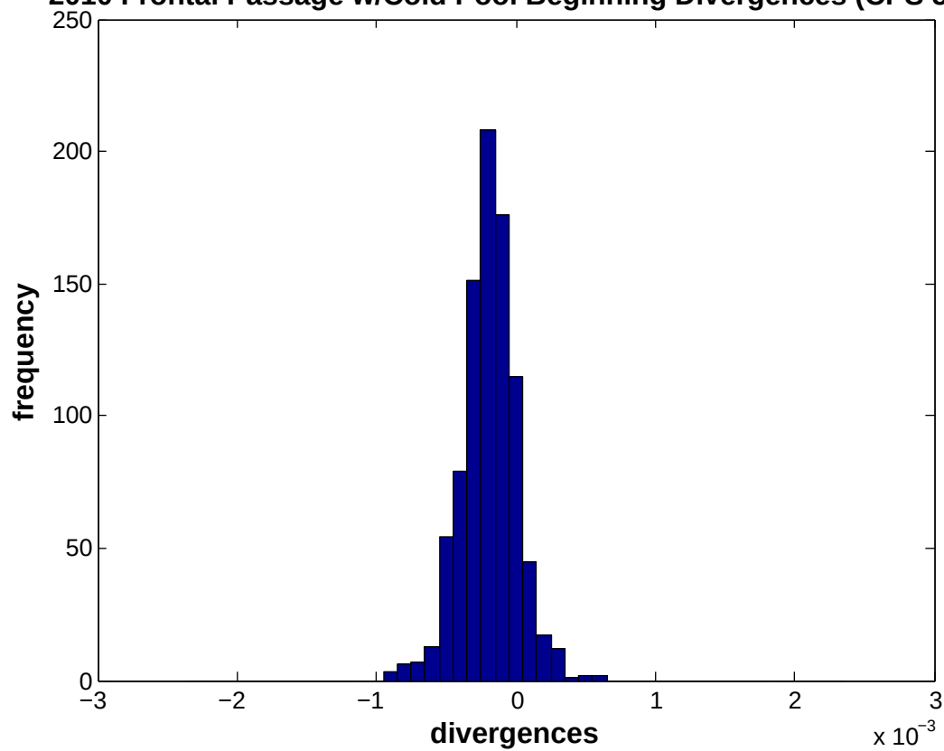
2010 Frontal Passage w/Cold Pool Beginning Divergences (CPS 5+)
