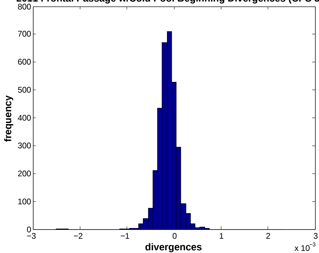
2011 Frontal Passage w/Cold Pool Beginning Divergences (CPS 3+)
