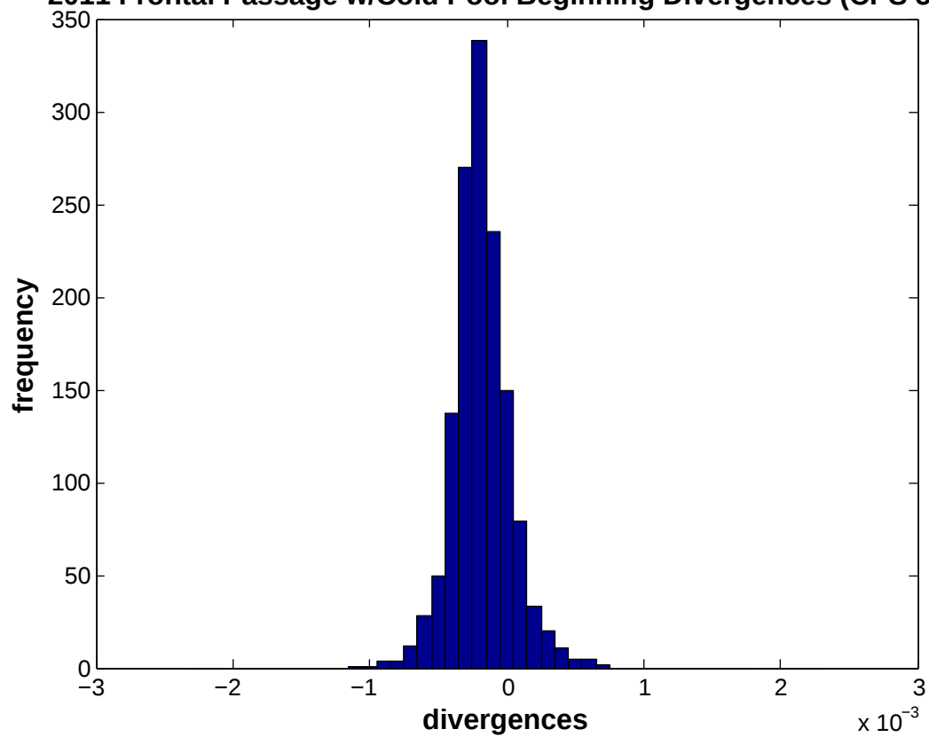
2011 Frontal Passage w/Cold Pool Beginning Divergences (CPS 5+)
