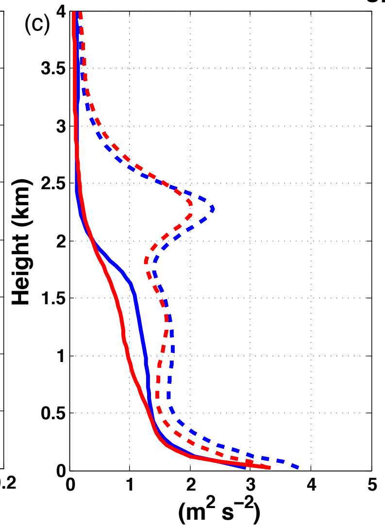
Total Turbulent Kinetic Energy
