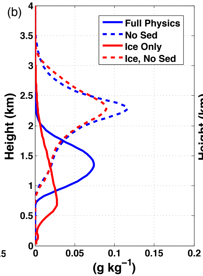
Total Cloud Water + Ice
