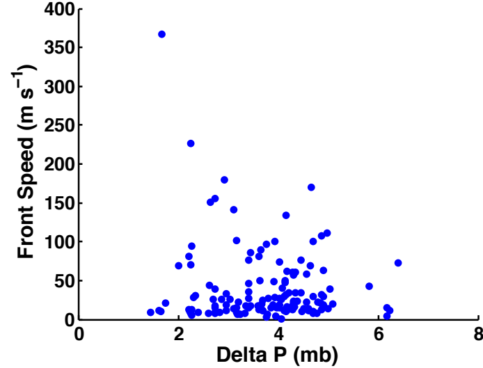
20 May 2011 8–20 UTC Case Frontal Passages
