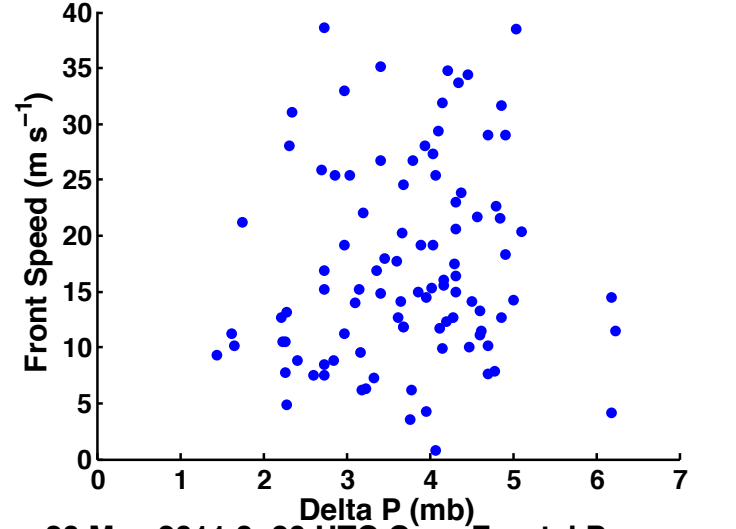
20 May 2011 8–20 UTC Case Frontal Passages
