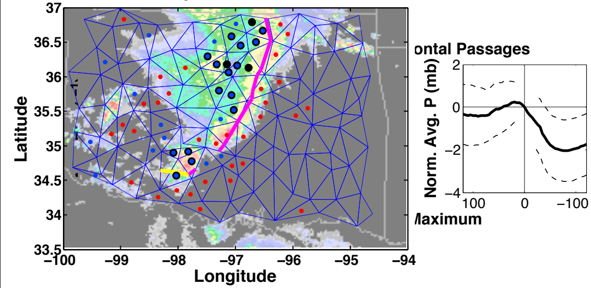
Cold Pool Analysis 1100 UTC 20 May 2011
