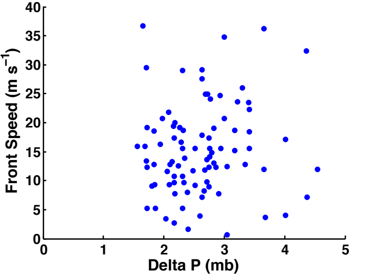
24–25 May 2011 18–6 UTC Case Frontal Passages
