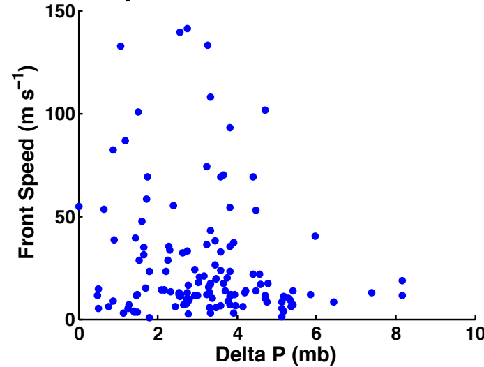
24–25 May 2011 18–6 UTC Case Frontal Passages
