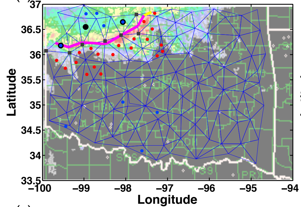
(c) Cold Pool Analysis 0300 UTC 16 June 2002
