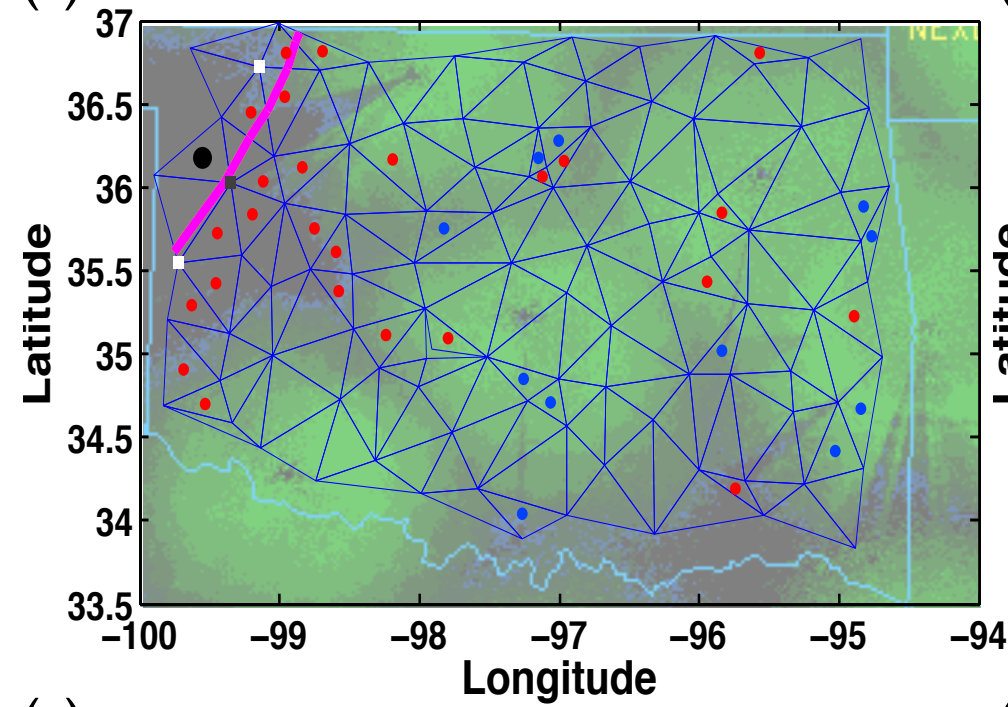
(c) Cold Pool Analysis 1100 UTC 30 April 2011
