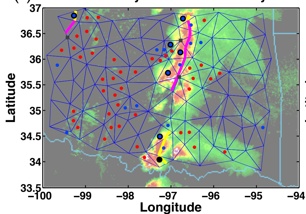
(c) Cold Pool Analysis 0000 UTC 25 May 2011
