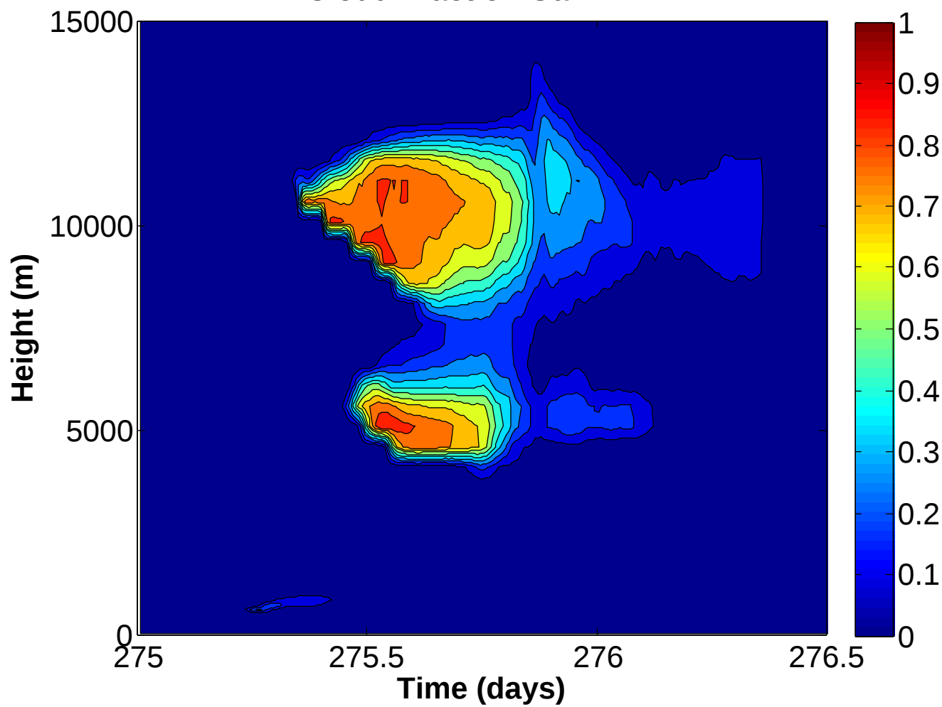
Cloud Fraction Gan 1km
