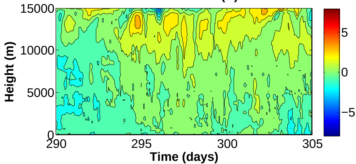
Model – Observed TABS (K) NSA 1km
