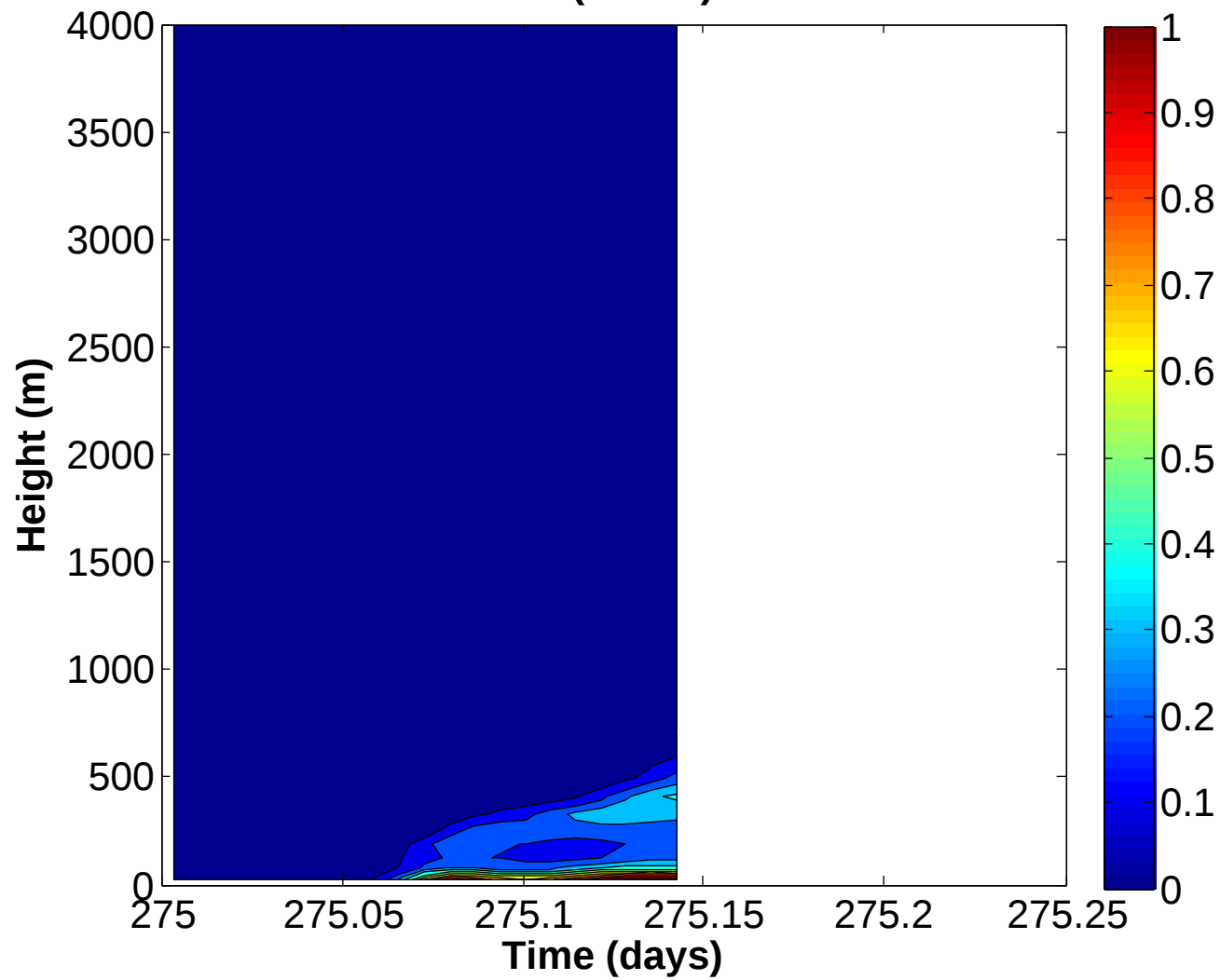
TKE Resolved ( \text{m}^2 \text{s}^{-2} ) Revelle 1km
