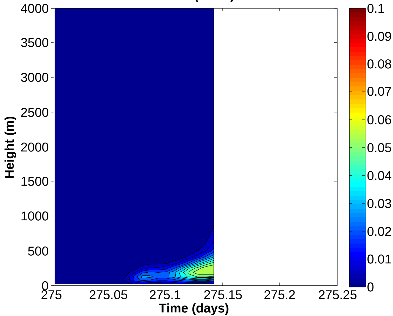
Vert. Vel. Variance ( \text{m}^2 \text{s}^{-2} ) Revelle 1km
