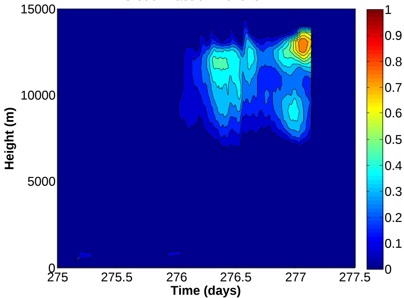
Cloud Fraction Revelle 1km
