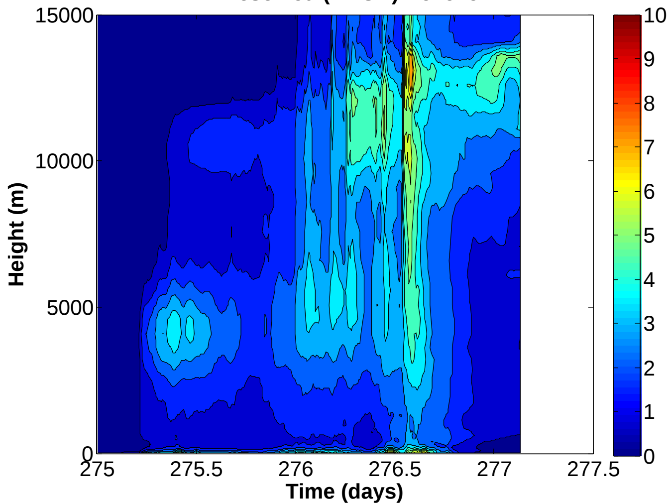
TKE Resolved ( \text{m}^2 \text{s}^{-2} ) Revelle 1km
