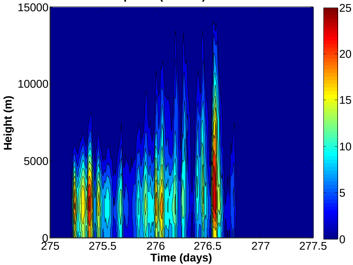
Precip Flux ( \text{mm d}^{-1} ) Revelle 1km
