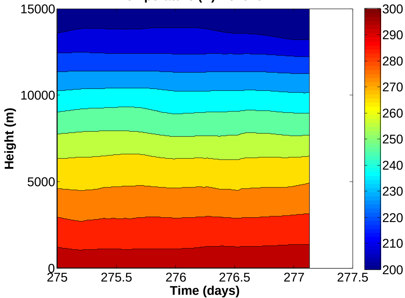
Temperature (K) Revelle 1km
