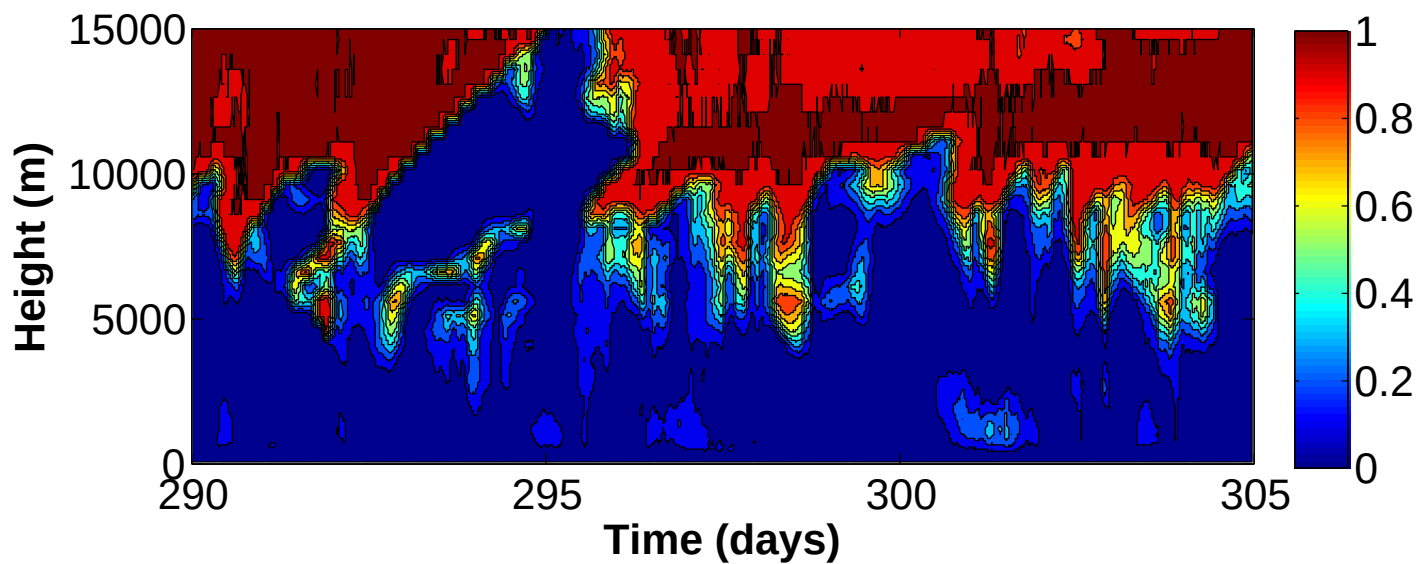
Cloud Fraction Revelle 1km
