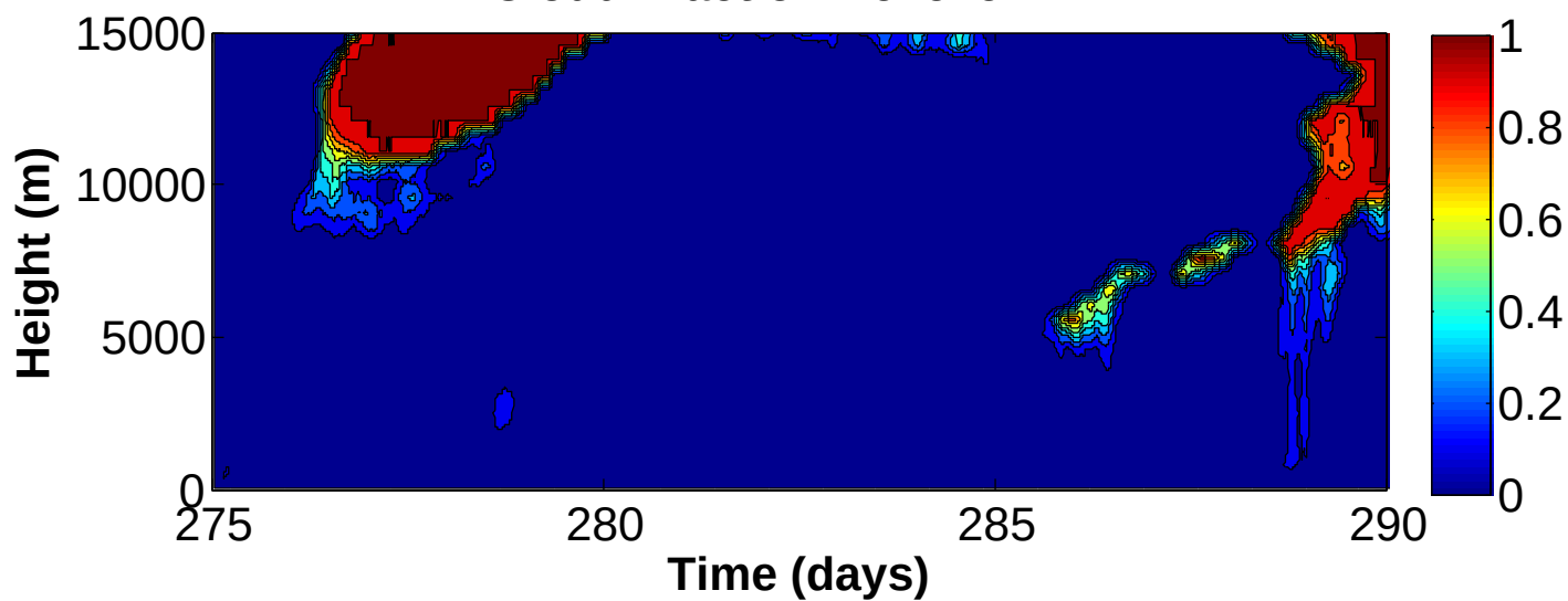
Cloud Fraction Revelle 1km
