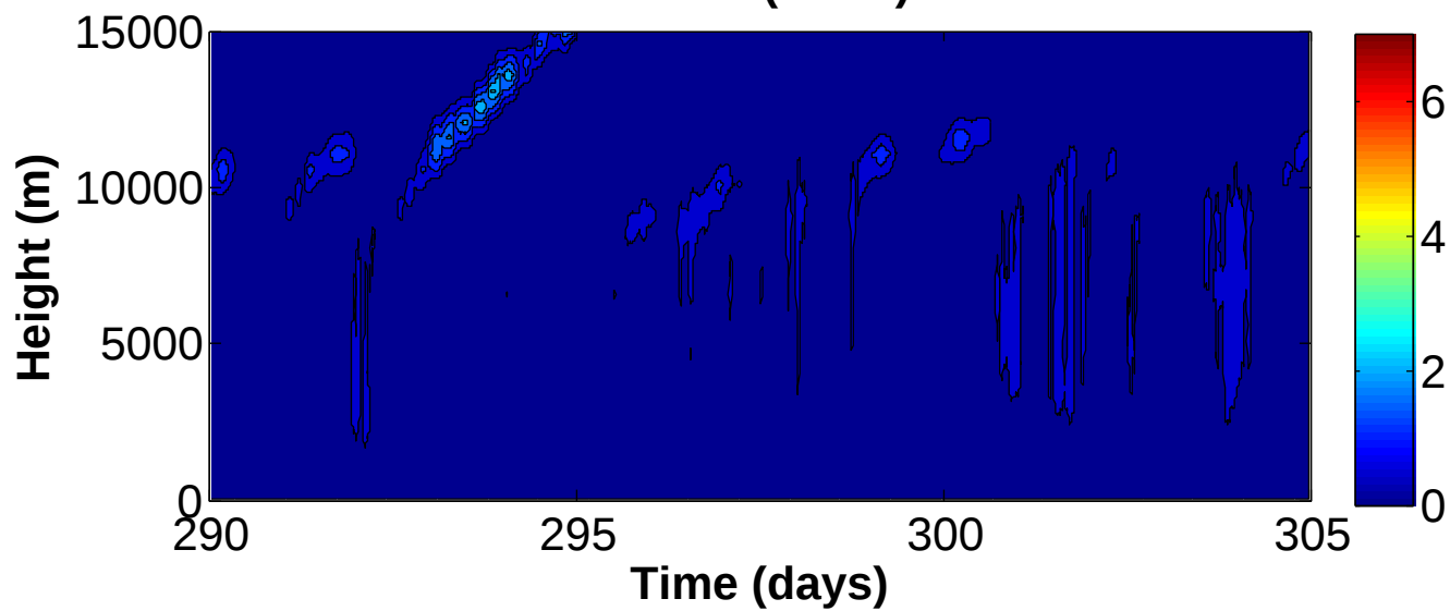
Vert. Vel. Variance ( \text{m}^2 \text{s}^{-2} ) Revelle 1km
