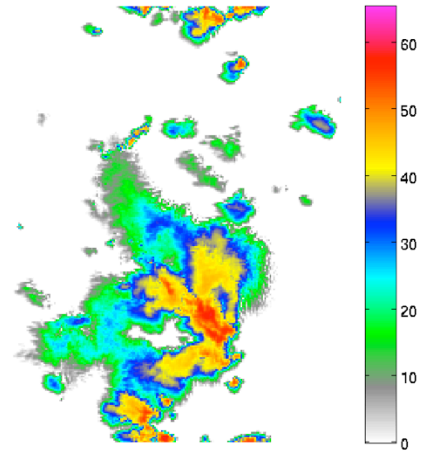
Precipitation (dbz) 0230z Oct. 21, 2011
