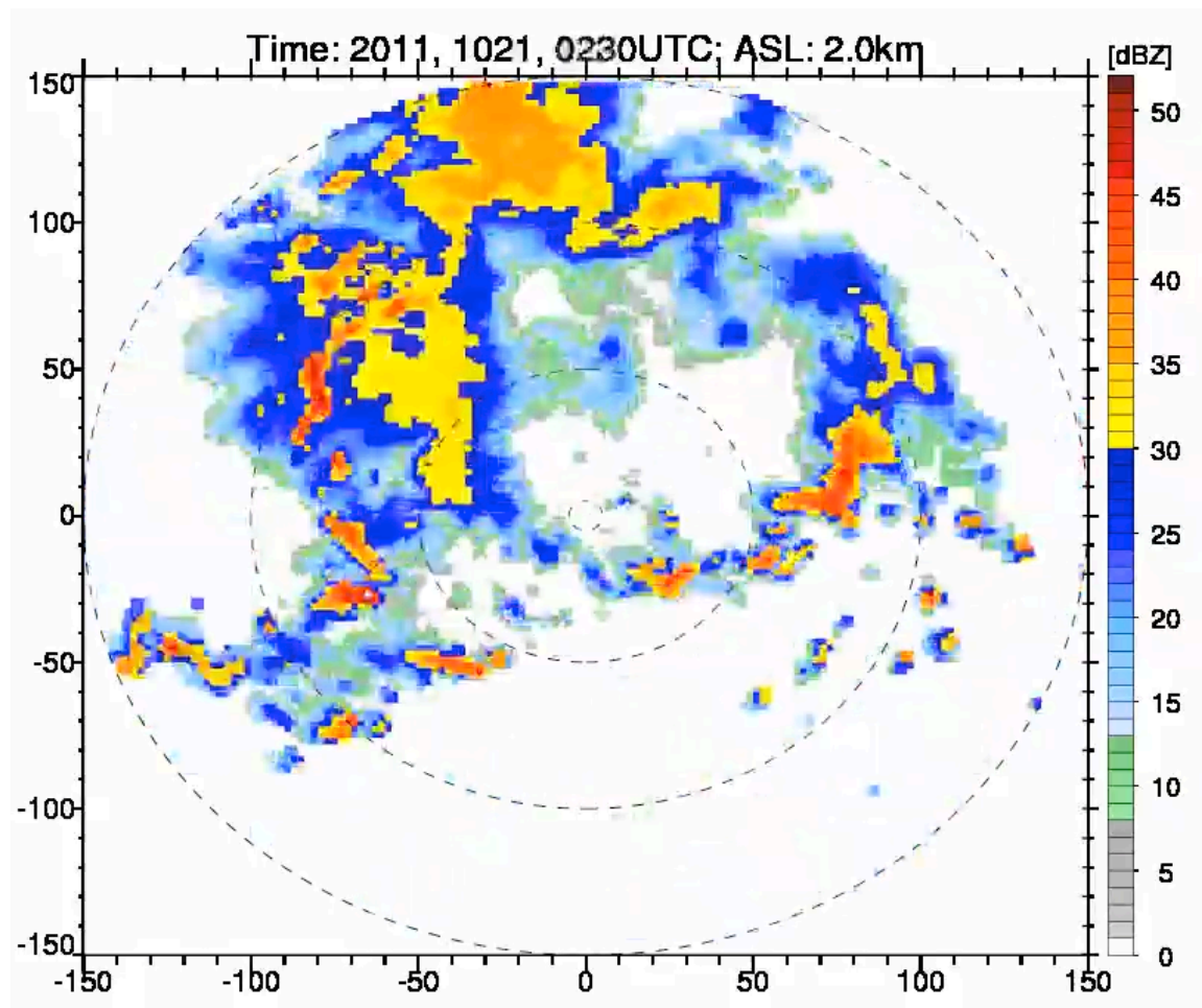
Precipitation (dbz) 0230z Oct. 21, 2011
