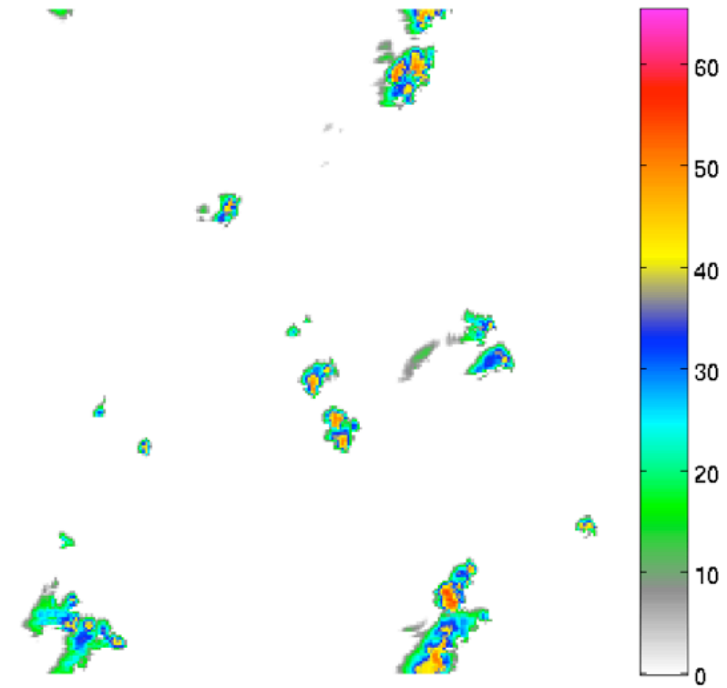
Precipitation (dbz) 2200z Oct. 16, 2011
