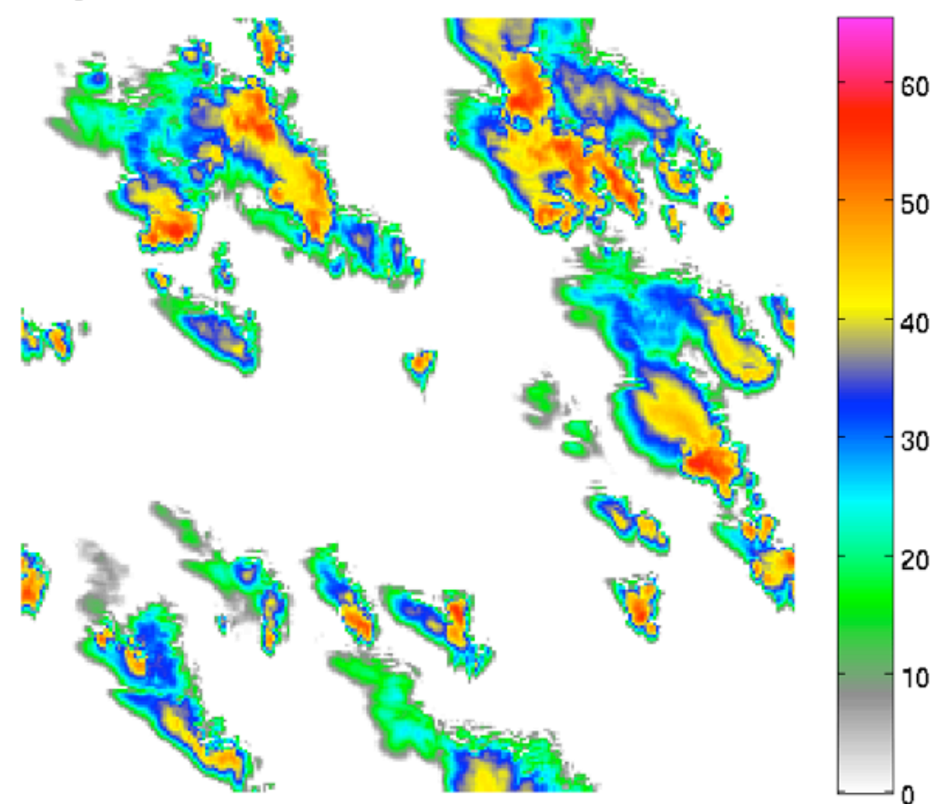
Precipitation (dbz) 1900z Oct. 27, 2011
