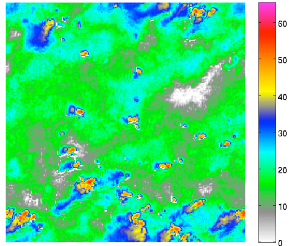
Precipitation (dbz) 1900z Oct. 29, 2011
