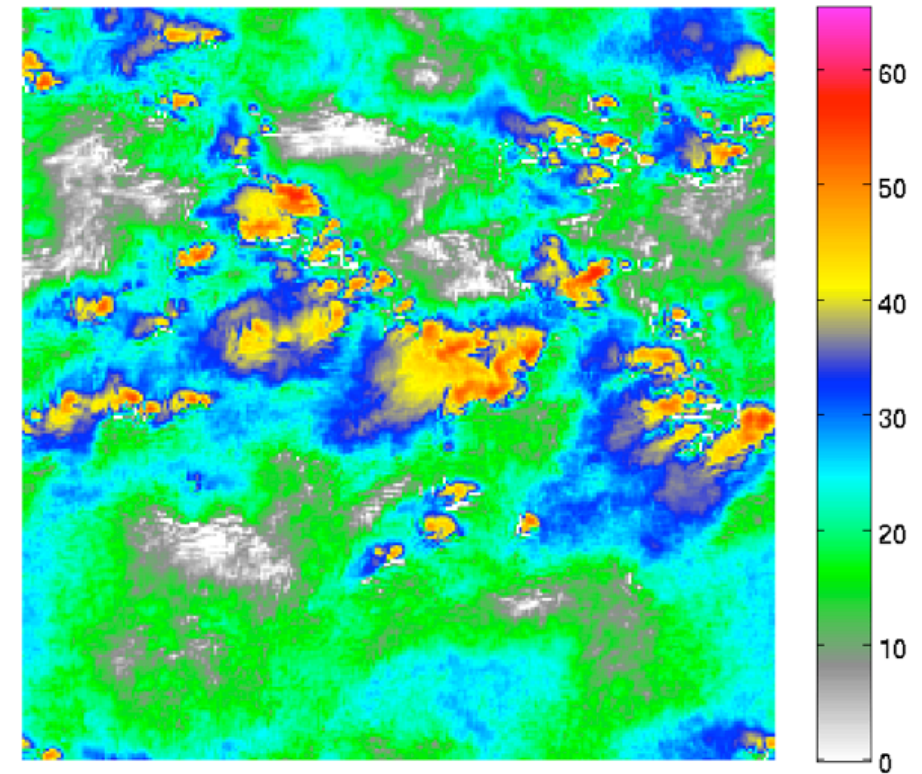
Precipitation (dbz) 1530z Oct. 29, 2011
