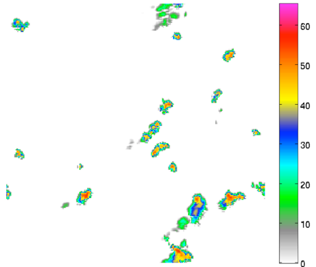
Precipitation (dbz) 0000z Oct. 17, 2011
