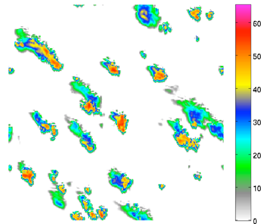
Precipitation (dbz) 1500z Oct. 27, 2011
