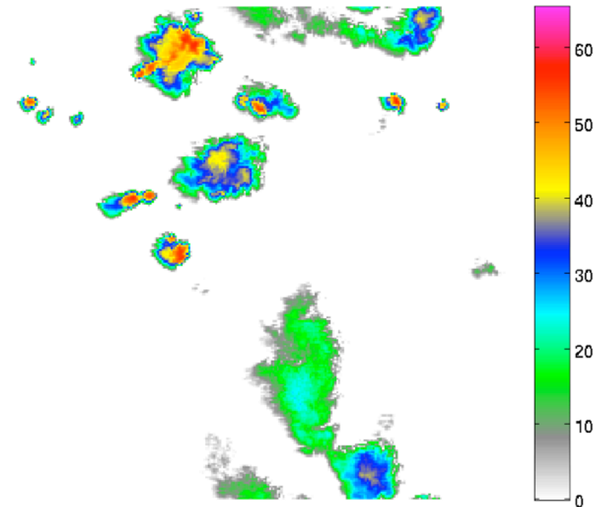
Precipitation (dbz) 0530z Oct. 21, 2011
