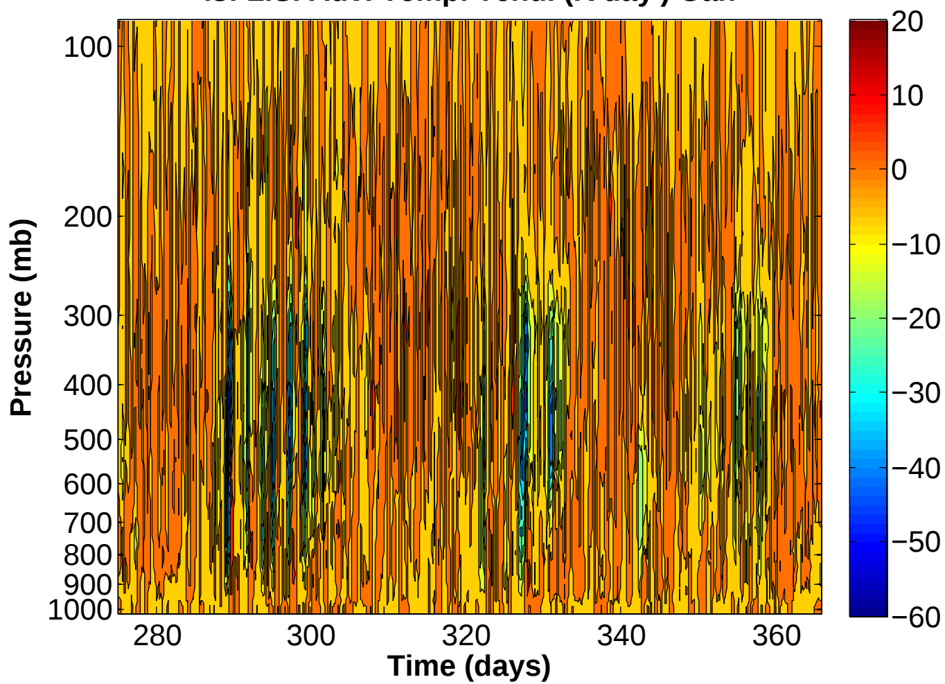
Isf L.S. Adv. Temp. Tend. ( \text{K day}^{-1} ) Gan
