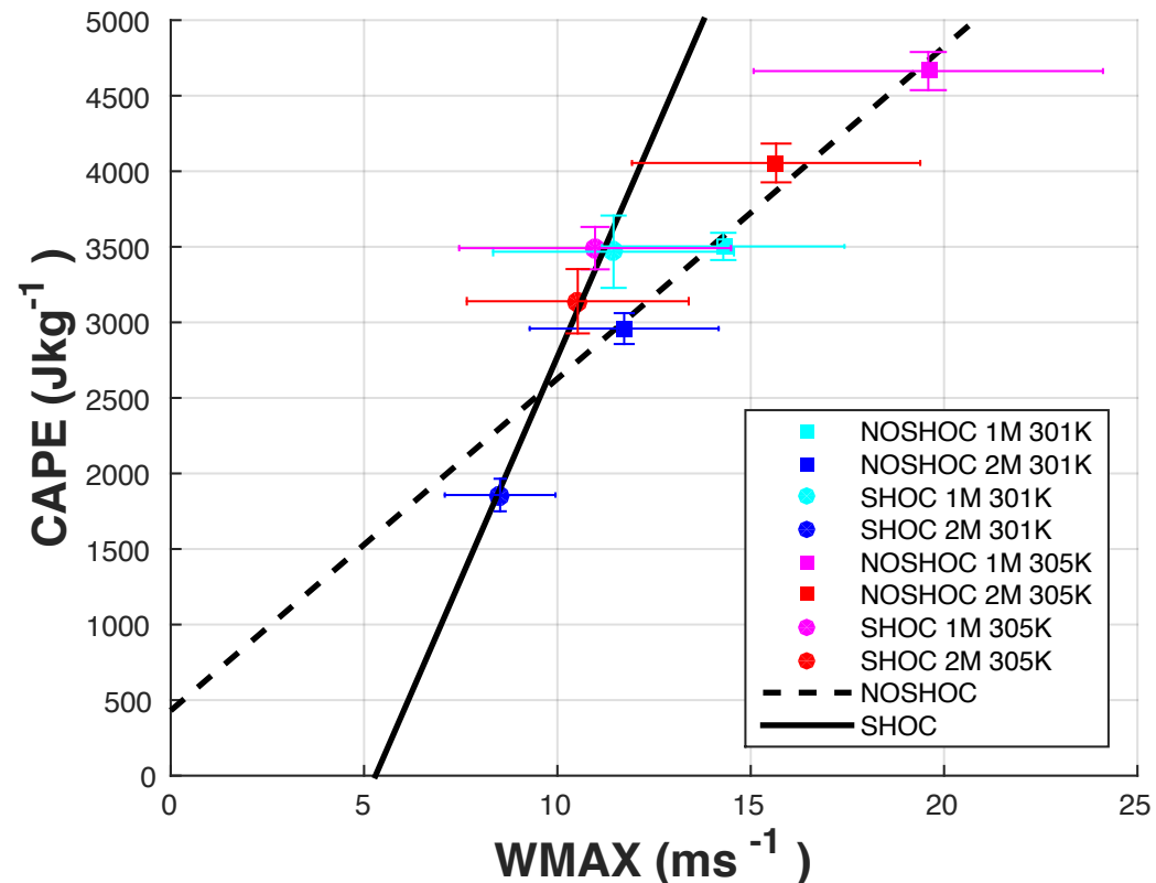
CAPE vs WMAX RCE-GREY 16km Runs
