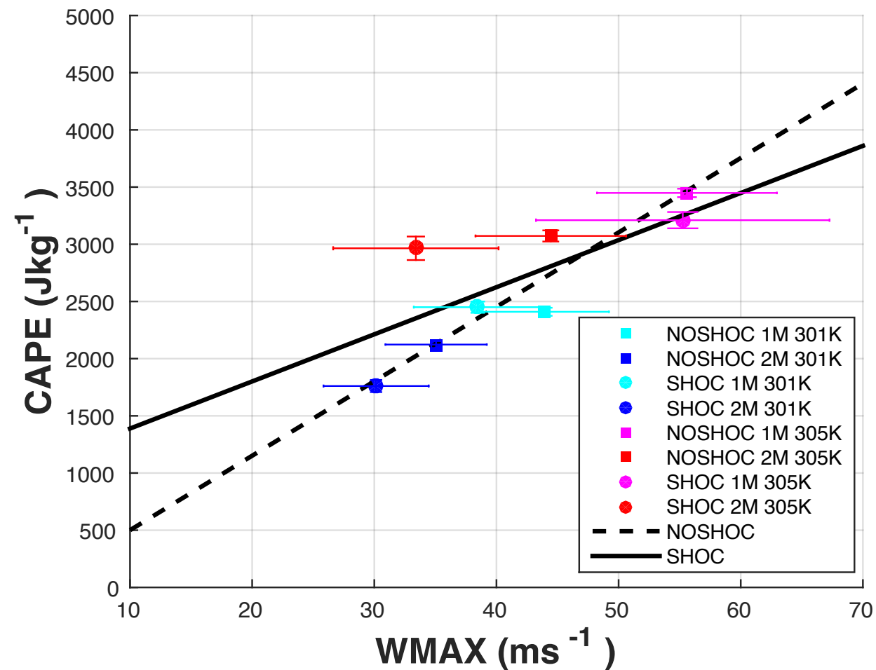
CAPE vs WMAX RCE-GREY 4km Runs
