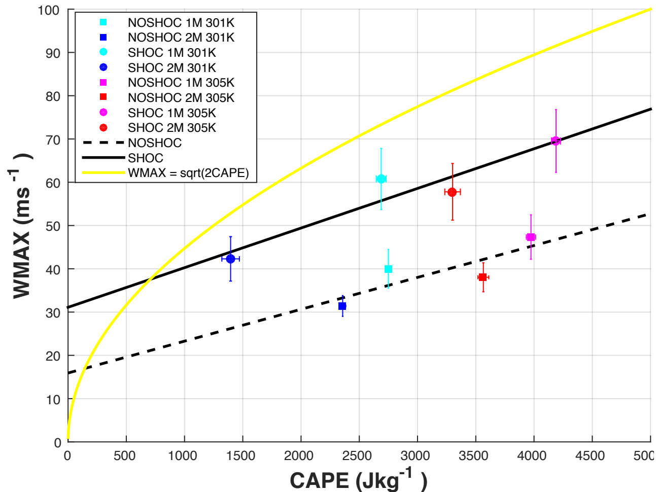
WMAX vs CAPE RCE-GREY 1km Runs
