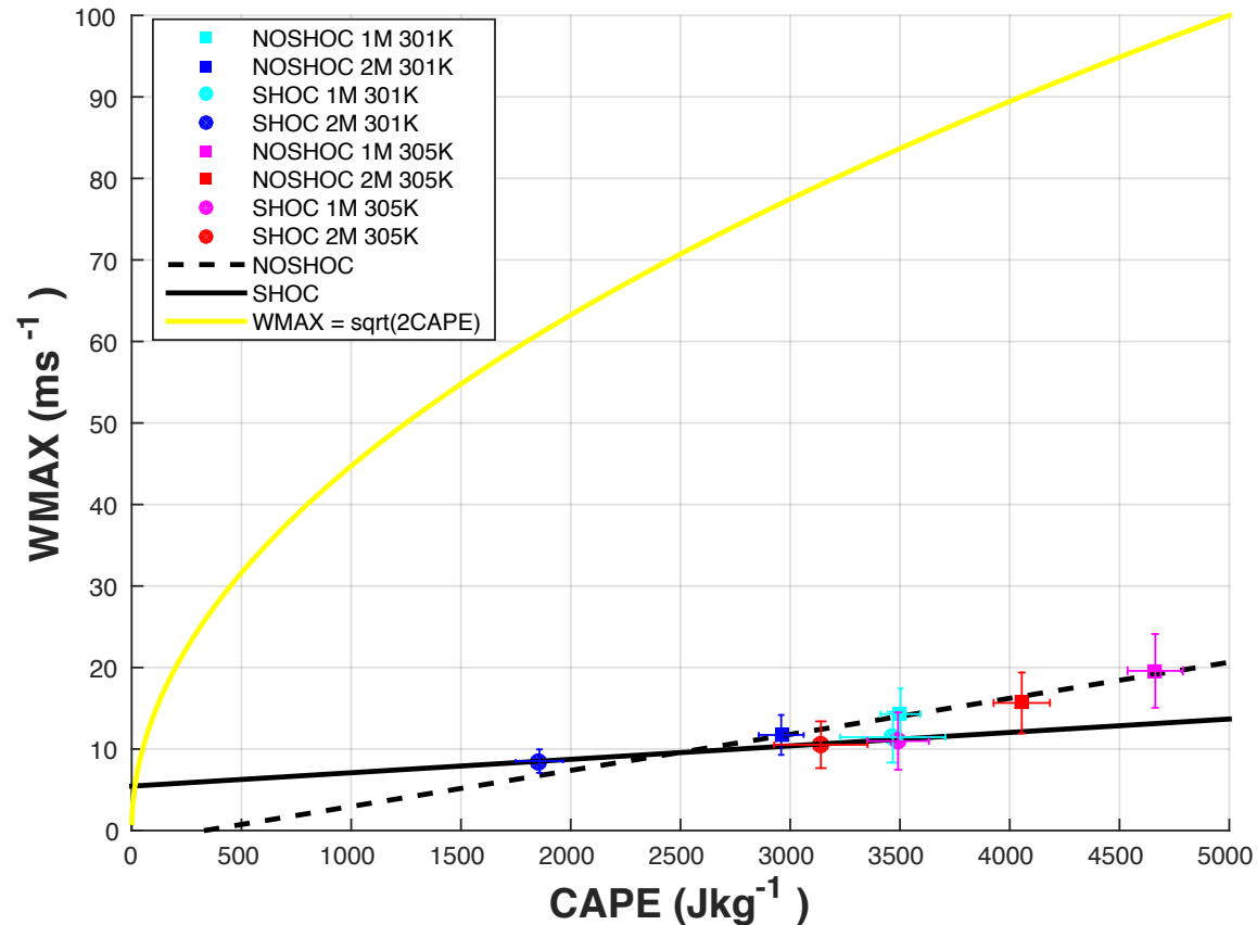
WMAX vs CAPE RCE-GREY 16km Runs
