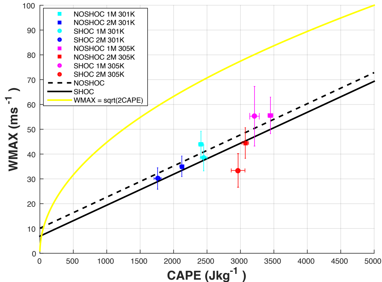
WMAX vs CAPE RCE-GREY 4km Runs
