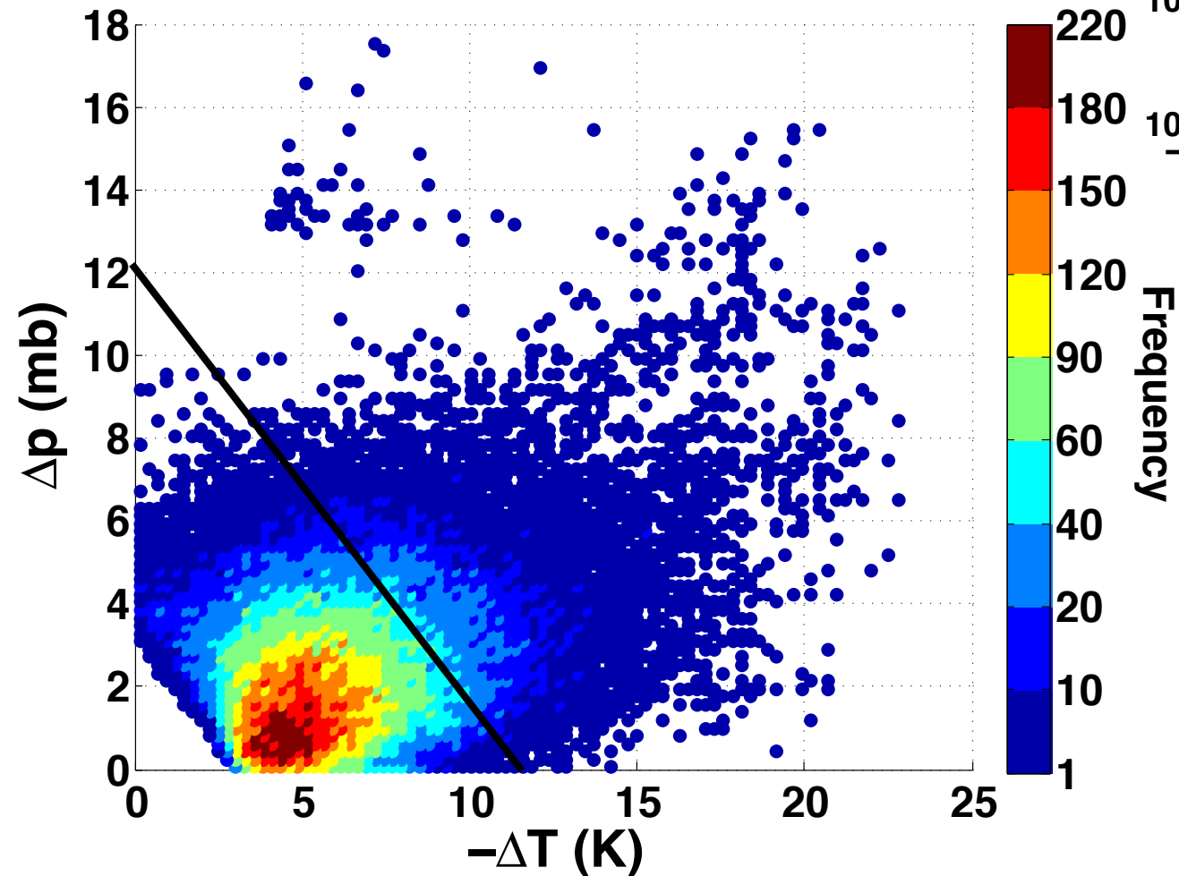
97-11 Frontal Passage -\Delta T and \Delta p (FS 3+)
