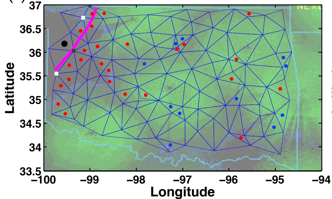
(c) Cold Pool Analysis 1100 UTC 30 April 2011
