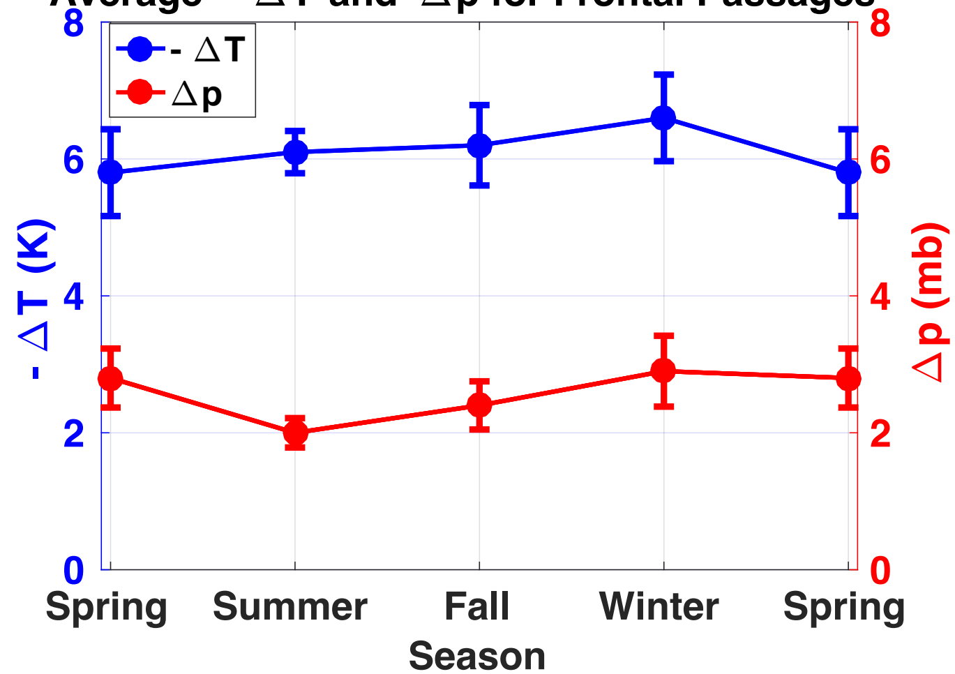
Average - \Delta T and \Delta p for Frontal Passages
