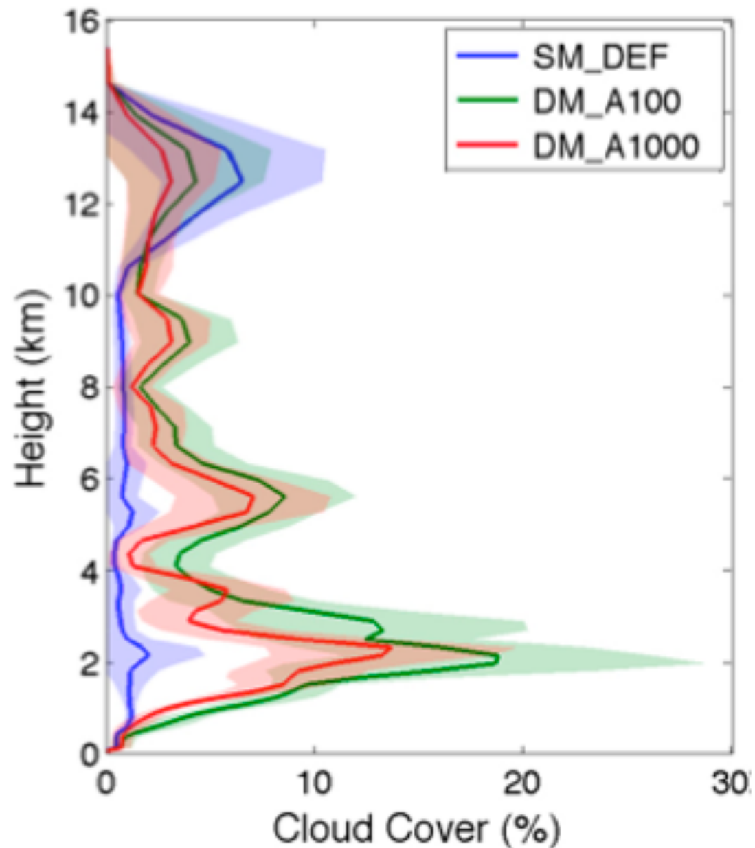
FIG. 3. Average cloud cover as a function of height in each of the three simulations. The shaded regions indicate one standard deviation in the time mean.
