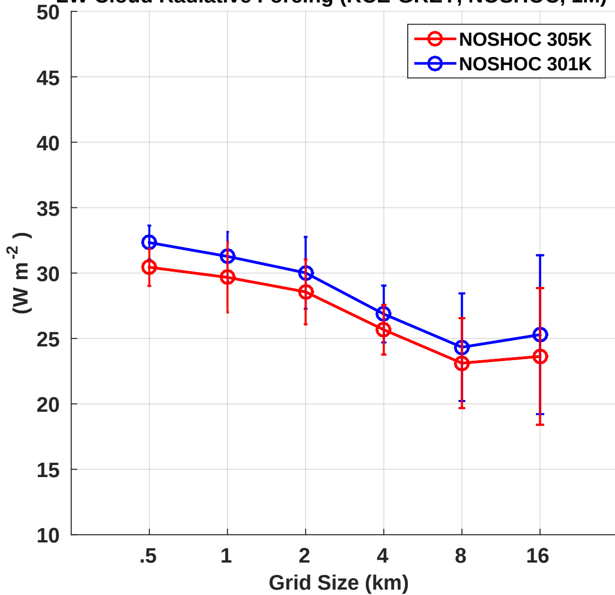
LW Cloud Radiative Forcing (RCE-GREY, NOSHOC, 1M)
