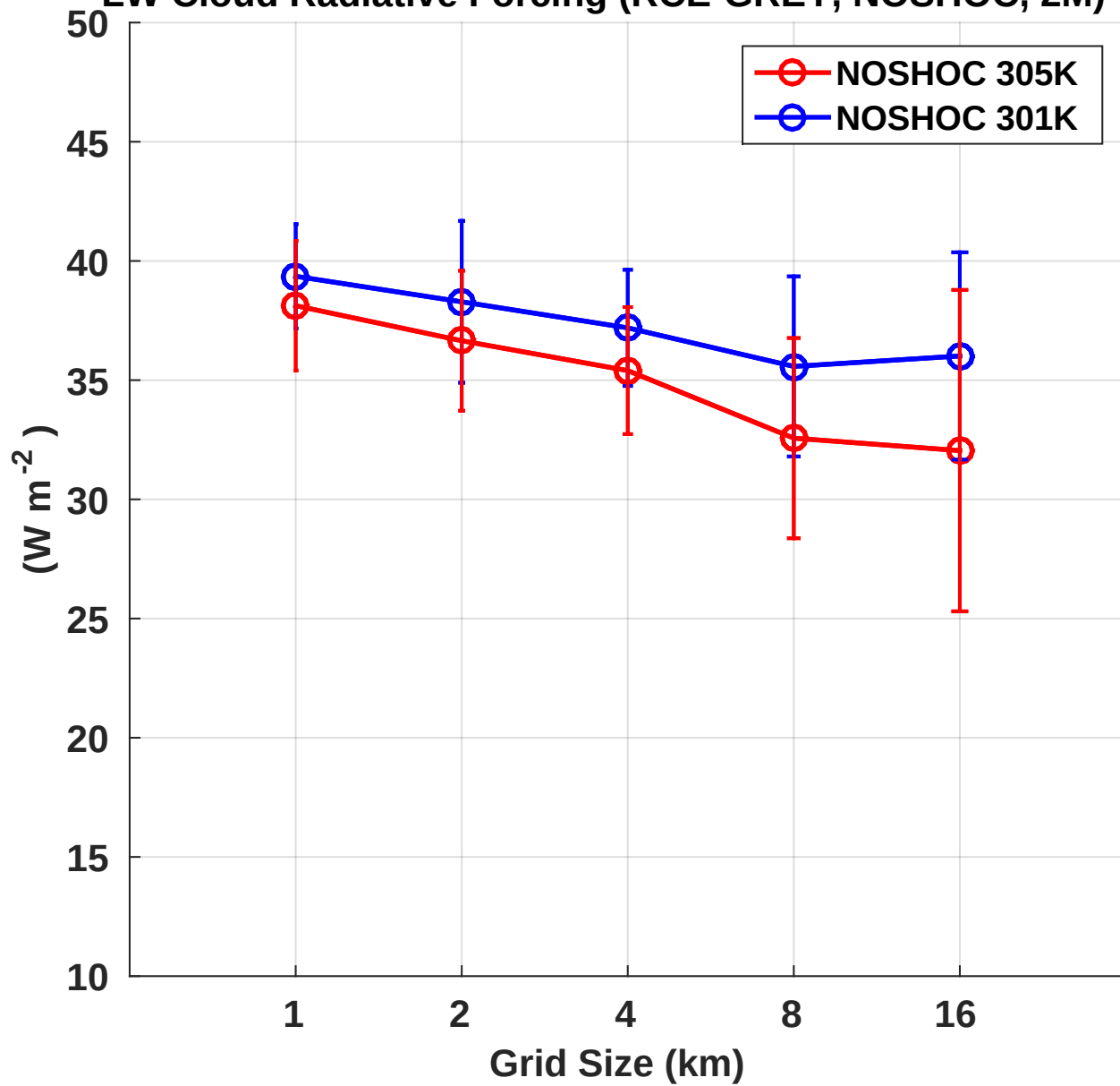
LW Cloud Radiative Forcing (RCE-GREY, NOSHOC, 2M)
