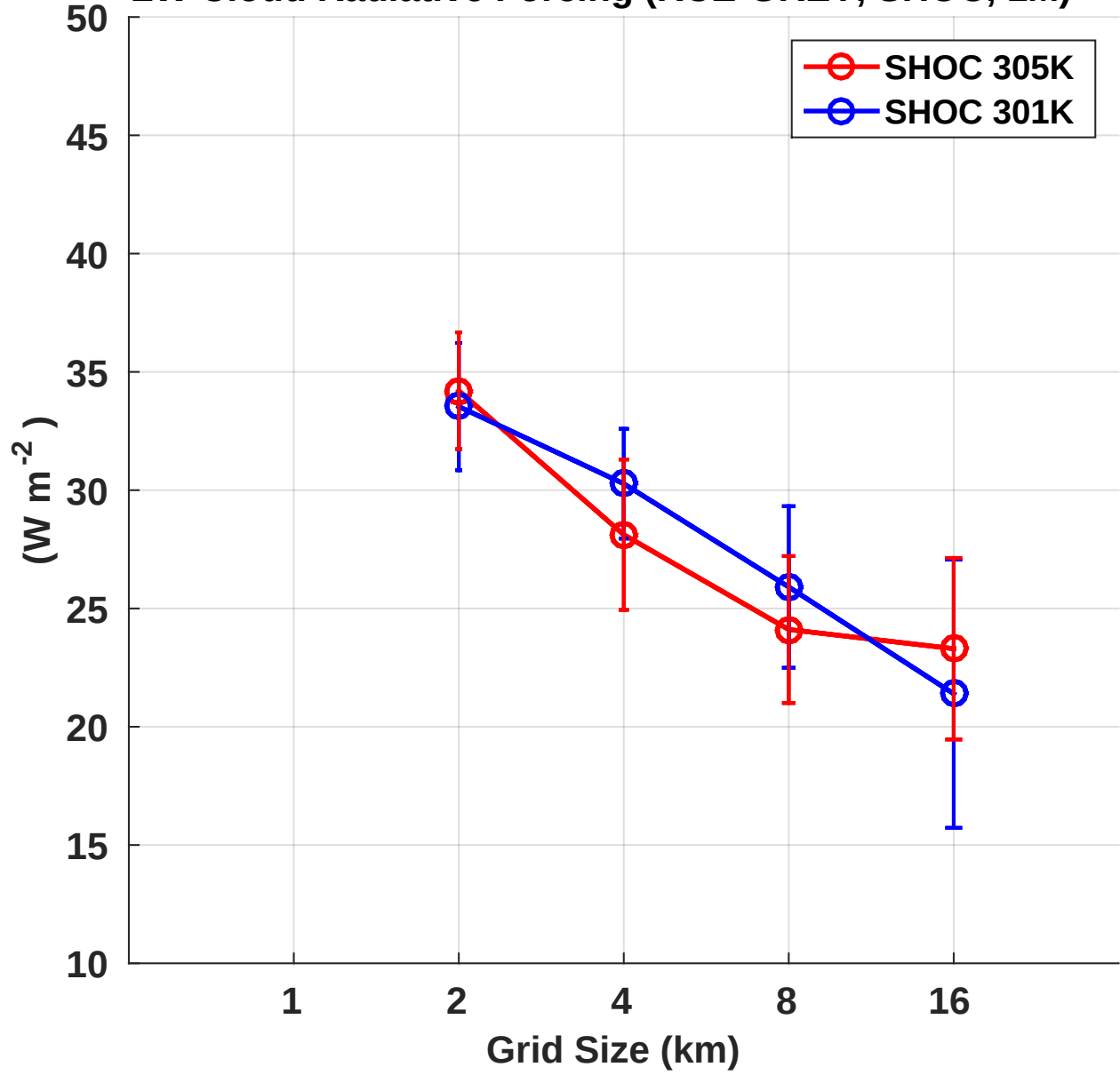
LW Cloud Radiative Forcing (RCE-GREY, SHOC, 1M)
