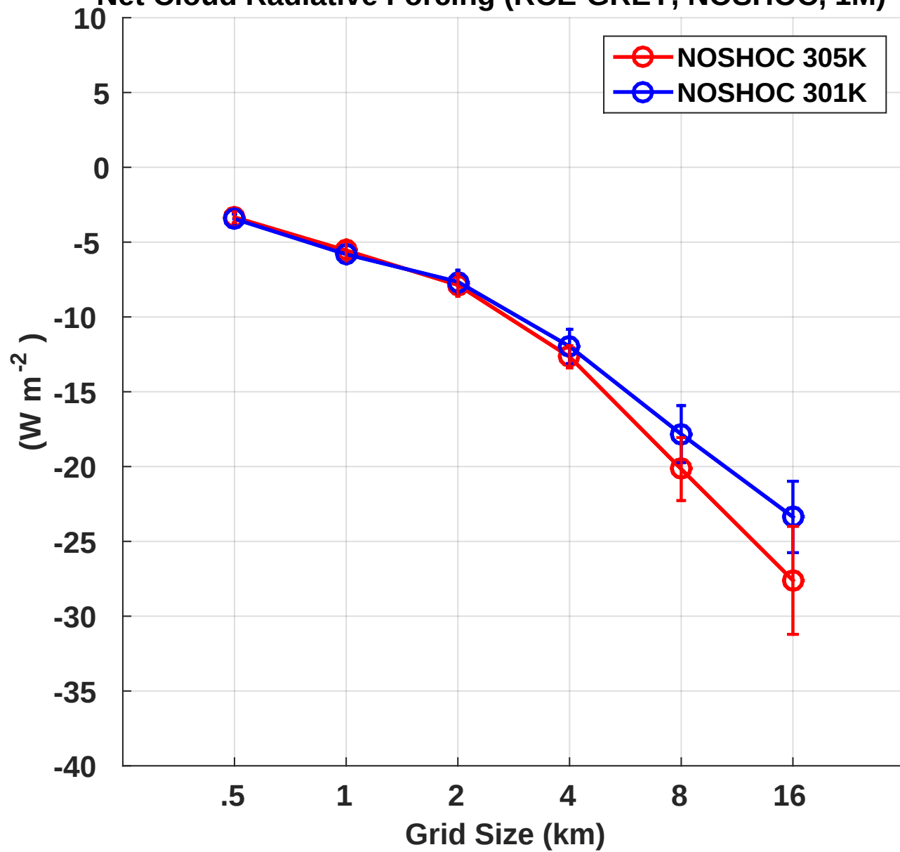
Net Cloud Radiative Forcing (RCE-GREY, NOSHOC, 1M)
