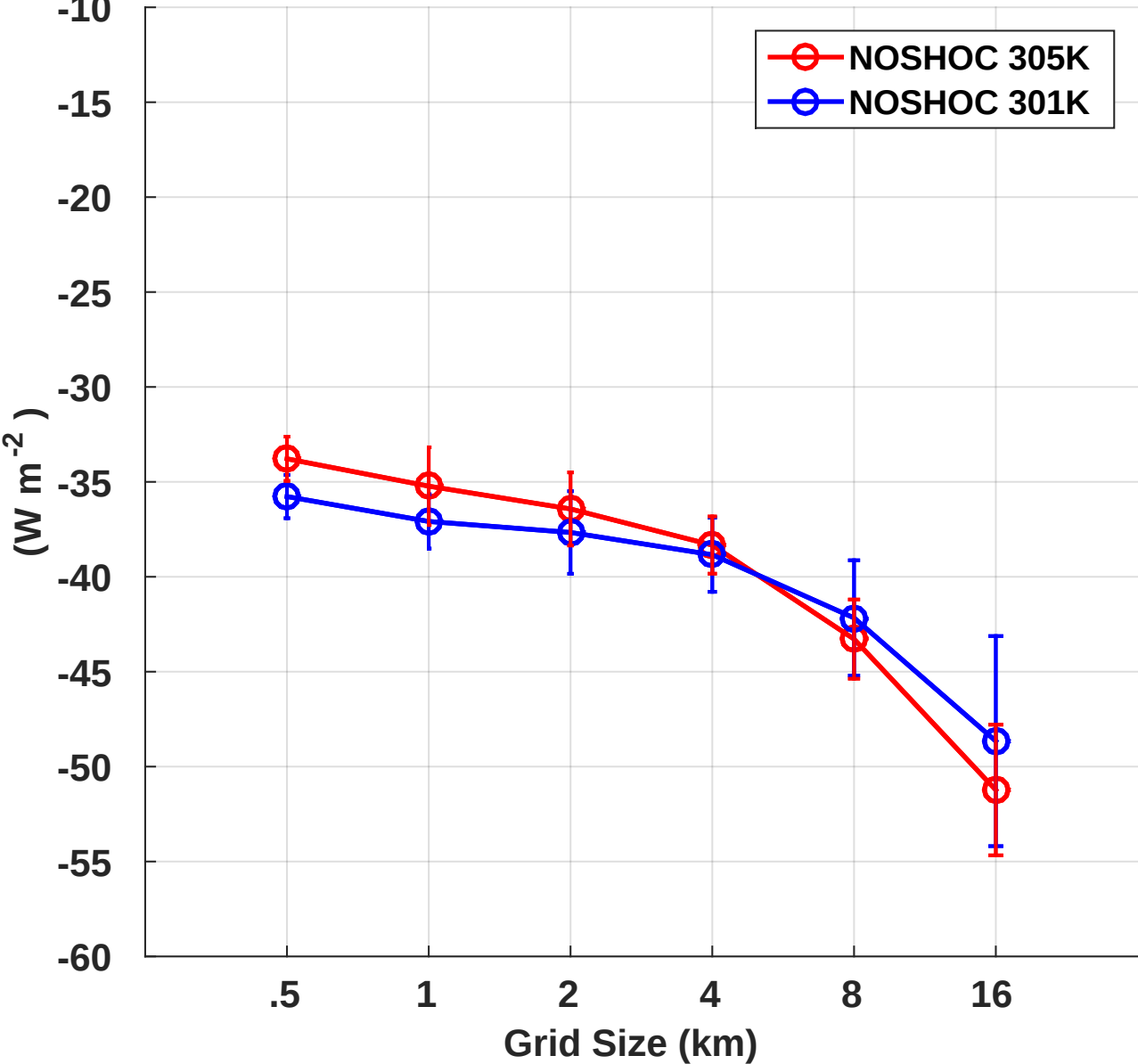
SW Cloud Radiative Forcing (RCE-GREY, NOSHOC, 1M)
