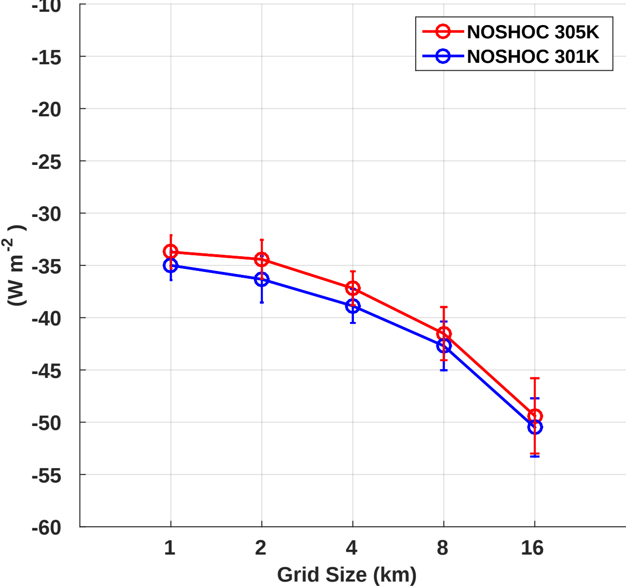
SW Cloud Radiative Forcing (RCE-GREY, NOSHOC, 2M)
