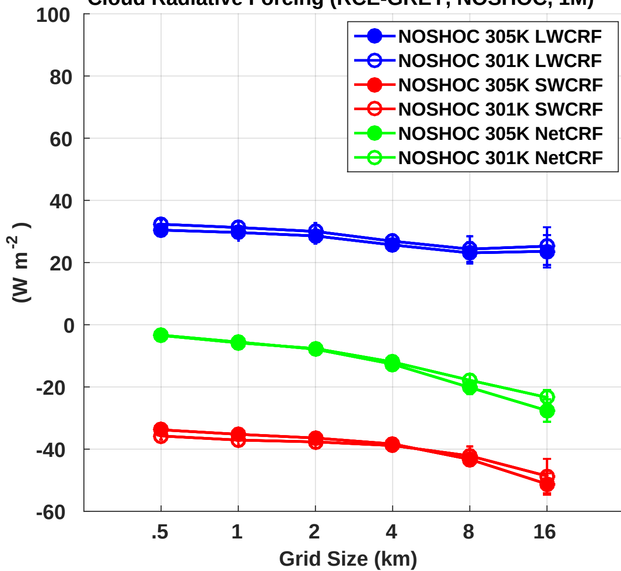
Cloud Radiative Forcing (RCE-GREY, NOSHOC, 1M)
