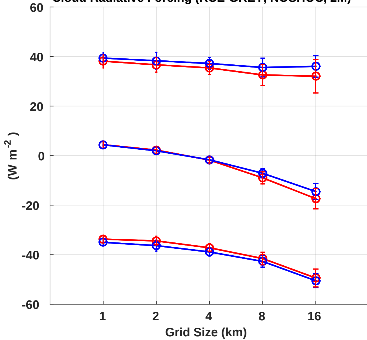
Cloud Radiative Forcing (RCE-GREY, NOSHOC, 2M)
