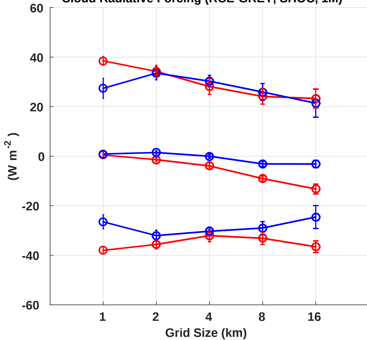
Cloud Radiative Forcing (RCE-GREY, SHOC, 1M)
