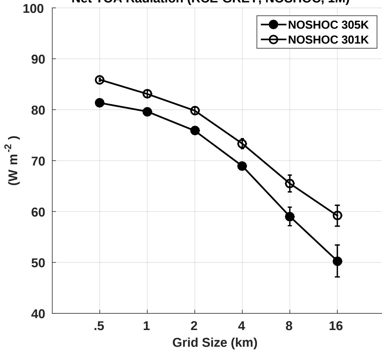
Net TOA Radiation (RCE-GREY, NOSHOC, 1M)
