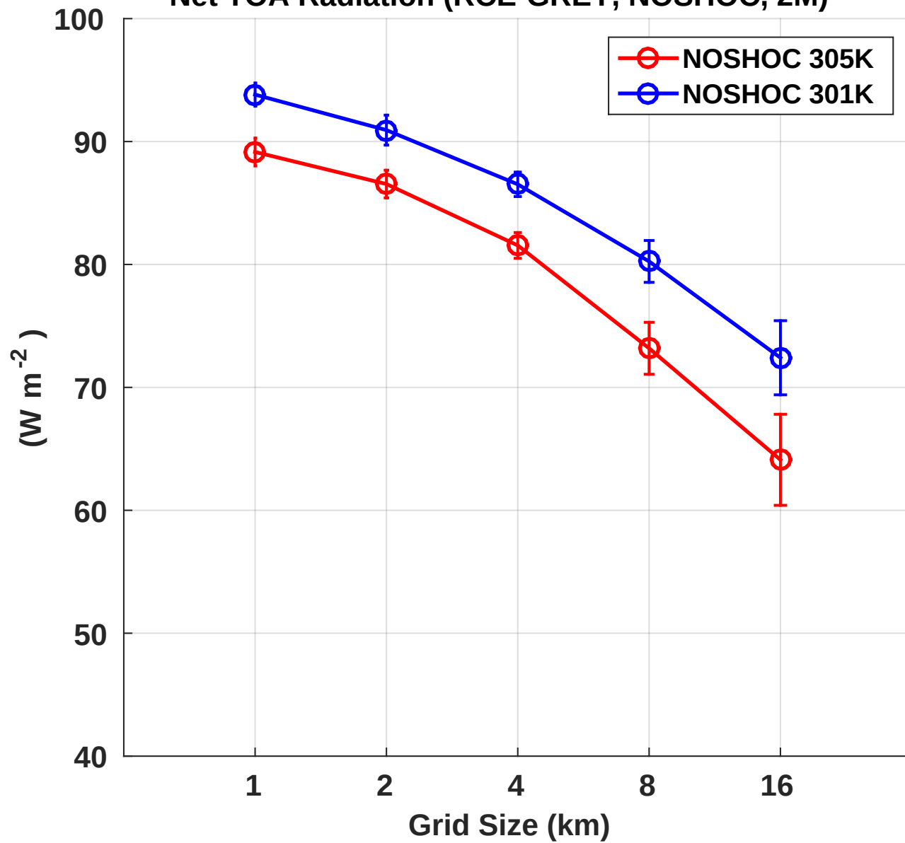
Net TOA Radiation (RCE-GREY, NOSHOC, 2M)
