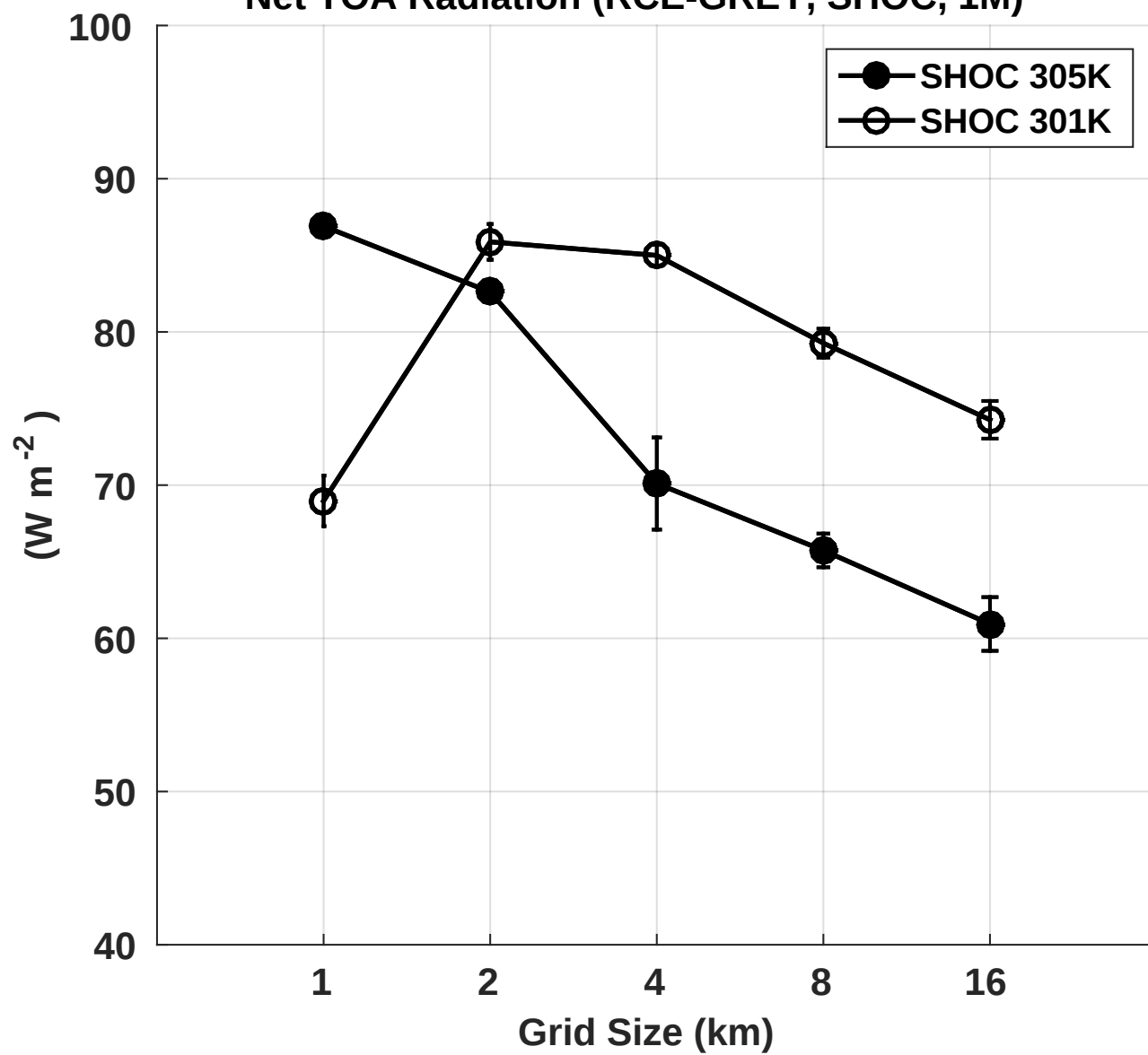
Net TOA Radiation (RCE-GREY, SHOC, 1M)
