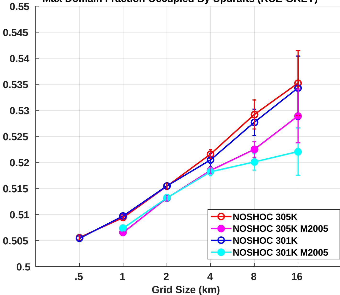
Max Domain Fraction Occupied By Updrafts (RCE-GREY)
