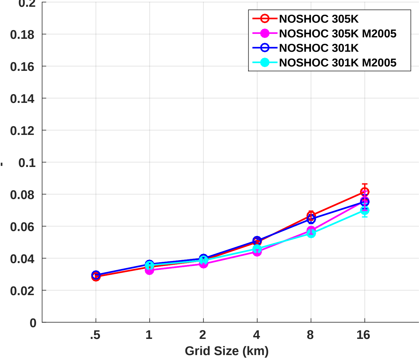
Max Cloud Fraction (RCE-GREY)
