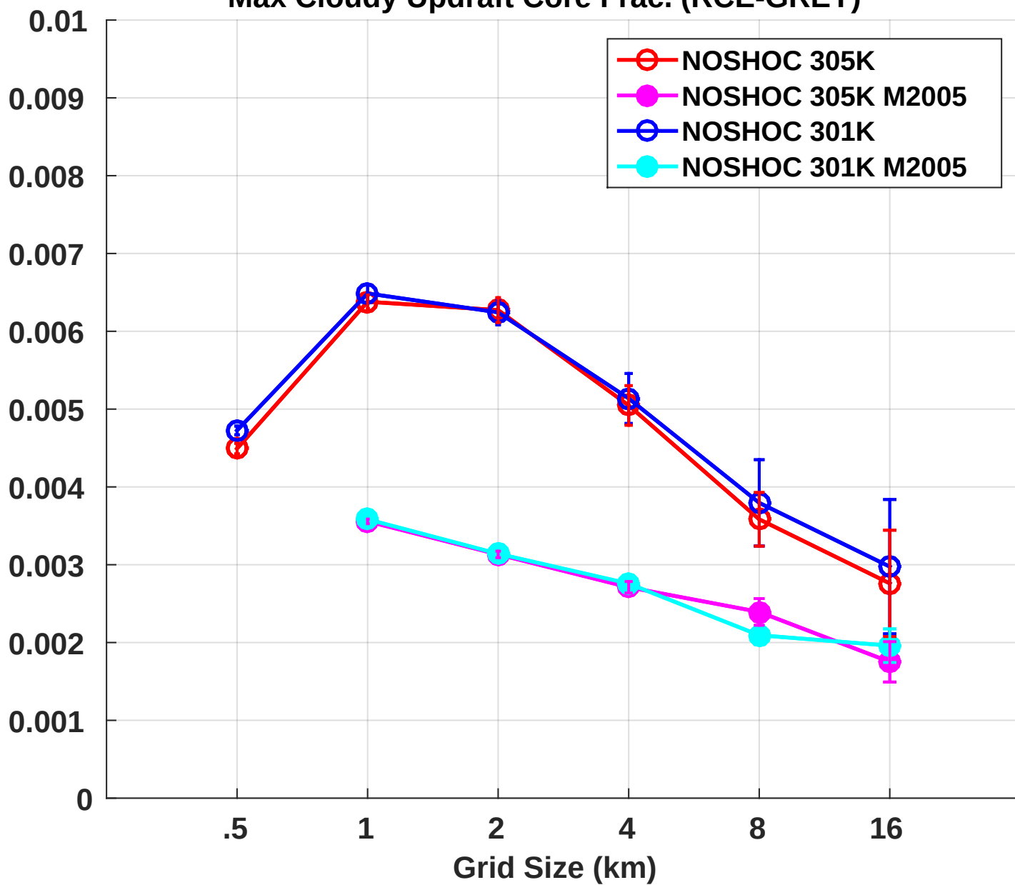
Max Cloudy Updraft Core Frac. (RCE-GREY)
