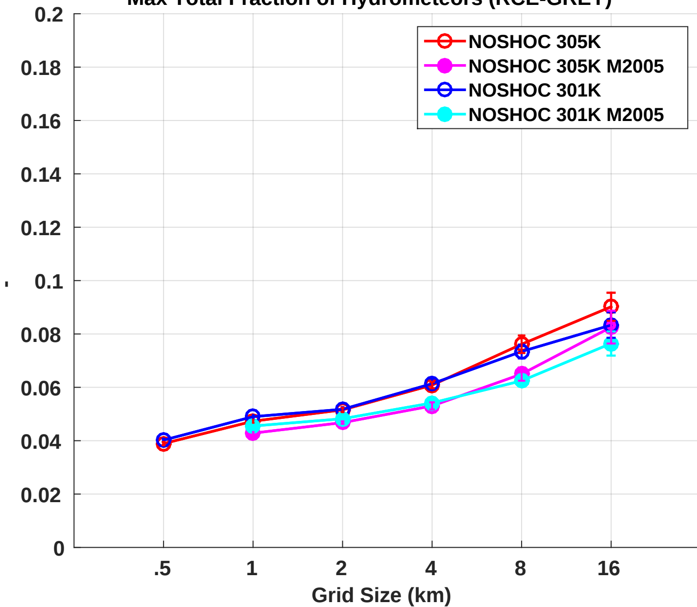
Max Total Fraction of Hydrometeors (RCE-GREY)
